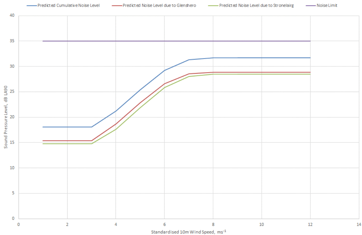
Chart 1: Cumulative Predicted Noise Levels & Noise Limits at Garvabeg (H41)
